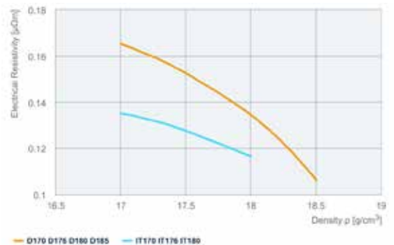
Electrical resistivity DENSIMET® and INERMET®
