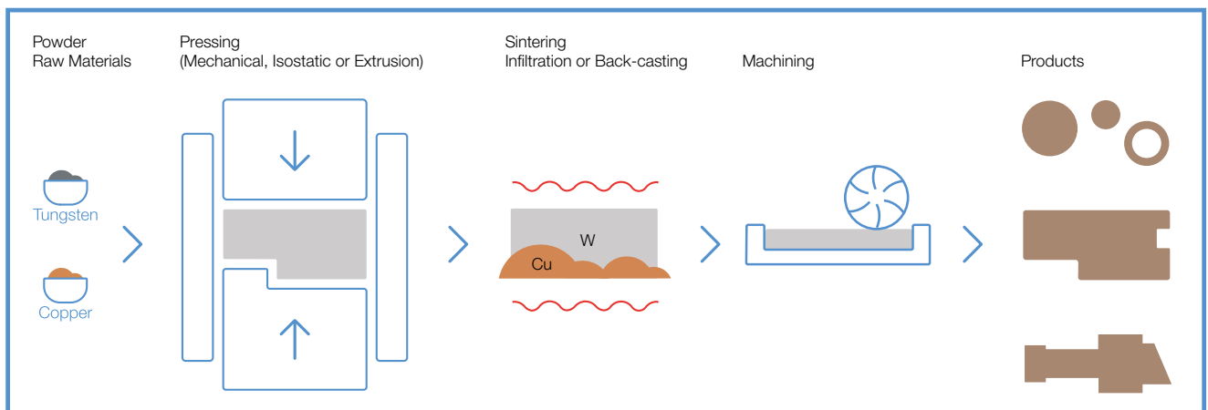
Figure 5: Schematic representation of the manufacturing process of WCu products and SPARKAL®
