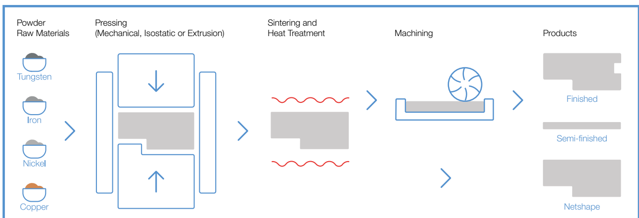
Figure 4: Manufacturing process of DENSIMET® and INERMET® products
